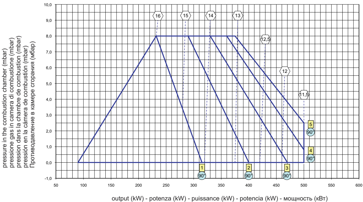
MAX GAS 500 PAB NATURAL GAS
