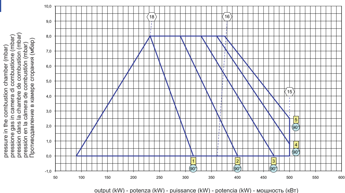
MAX GAS 700 PAB NATURAL GAS / LPG
