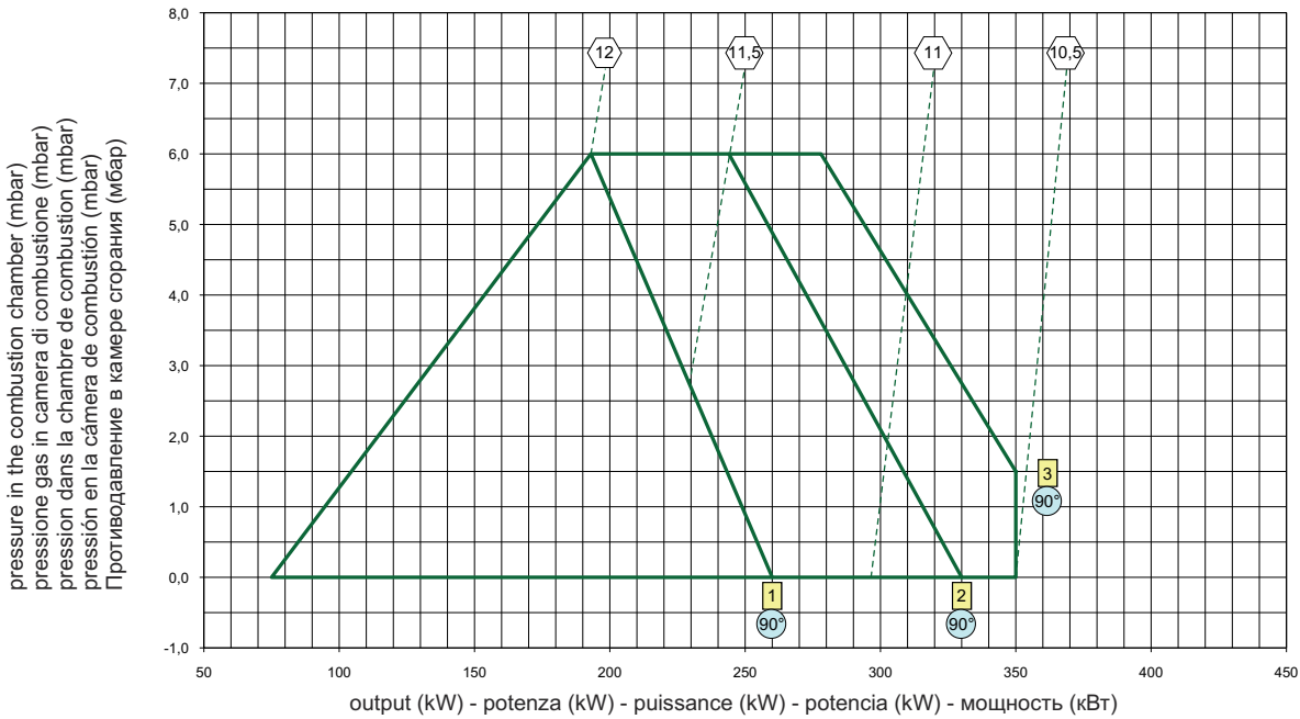
MAX GAS 350 PAB NATURAL GAS / LPG
